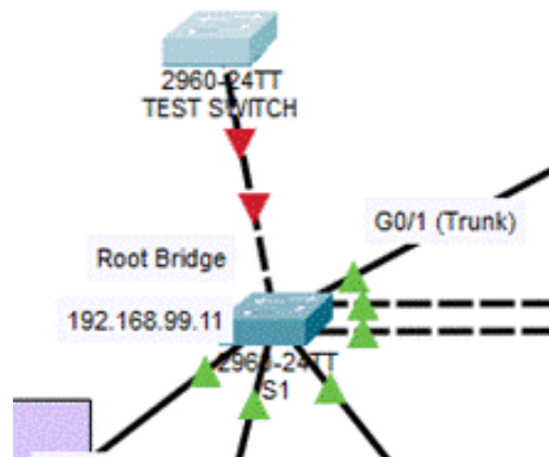
Figure 7.18.1: T13 (Packet Tracer) - TEST SWITCH connected to S1 Fa0/2 to generate BPDUs. The link is shown red because BPDUGuard has already err-disabled the port.
