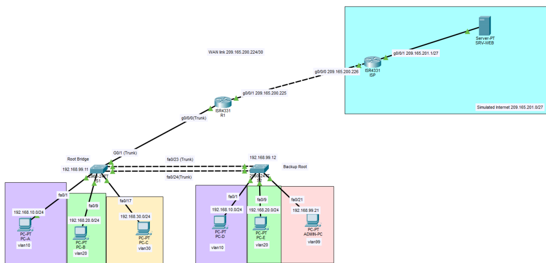
Figure 4.2: Logical network topology for the Packet Tracer implementation.
