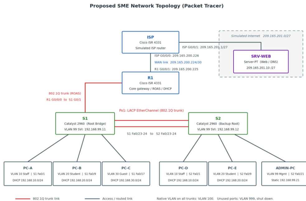
Figure 4.1: Proposed network topology for the Packet Tracer implementation.
