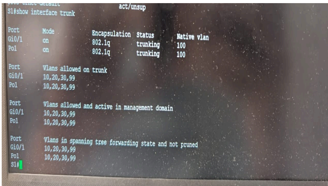
Figure 7.10: T8 - show interfaces trunk on S1
