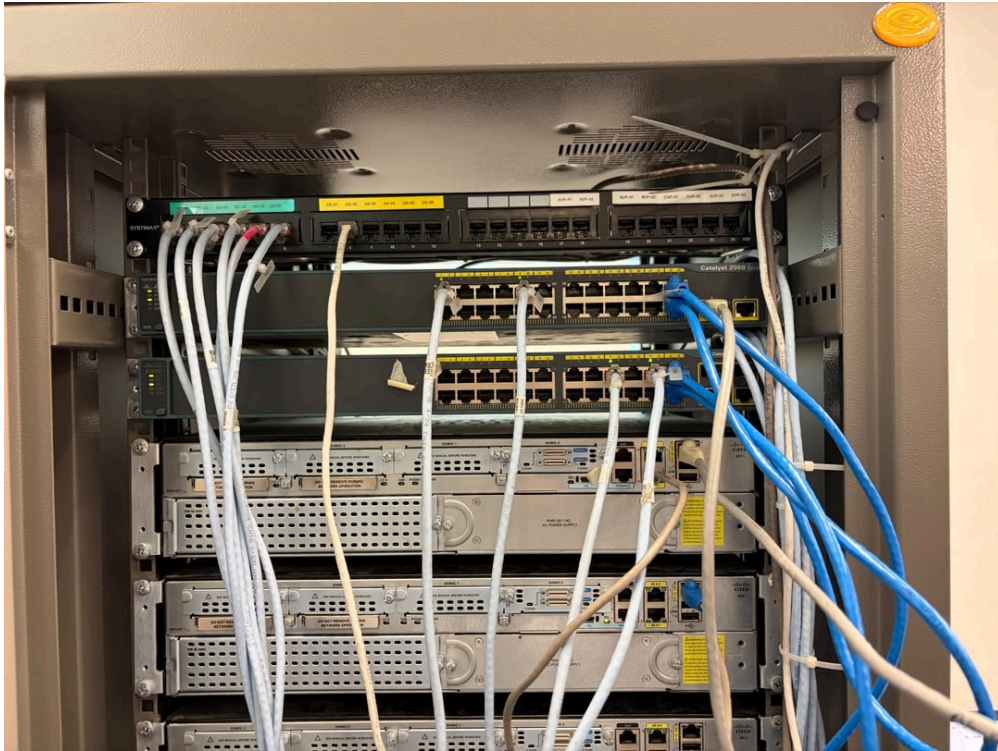
Figure 4.3: Physical network topology for the Lab implementation.
