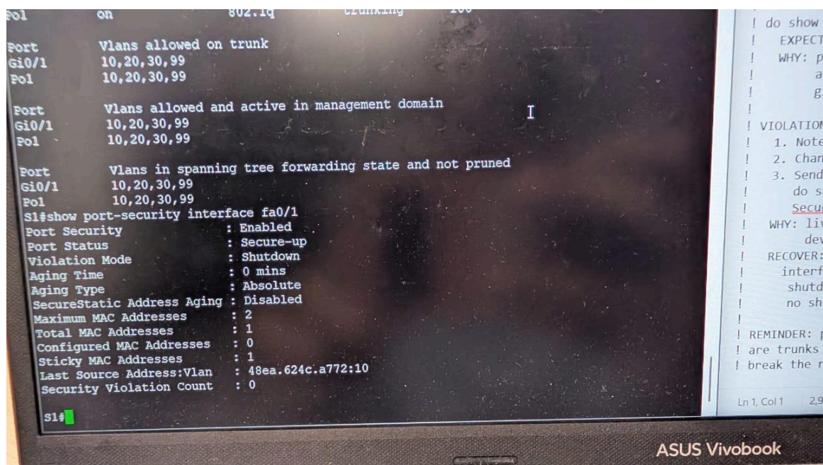
Figure 7.15.1: T12 - show port-security interface fa0/1 BEFORE violation
